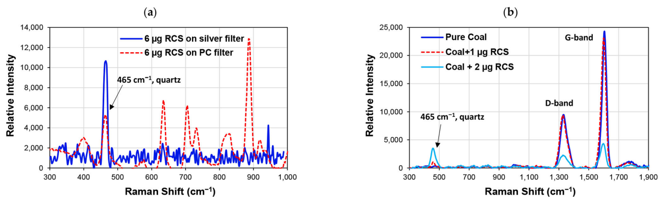
Figure 6. Raman spectra for: (a) crystalline silica on silver-membrane and polycarbonate (PC)-membrane filters; and (b) samples of pure coal and coal mixed with 1 \mu\text{g} and 2 \mu\text{g} of RCS on a PC filter.
