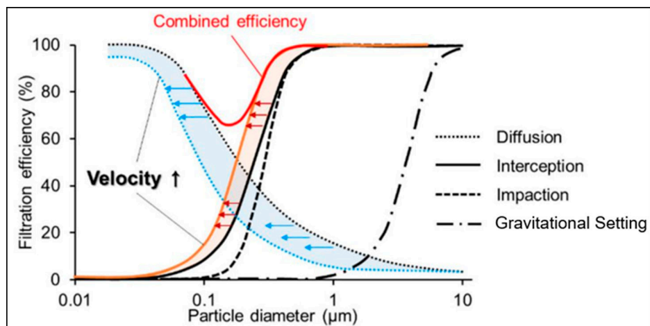
Figure 1. Illustration of the combined effects of the particle capture mechanisms for solid particles on the overall filtration efficiency [12].
