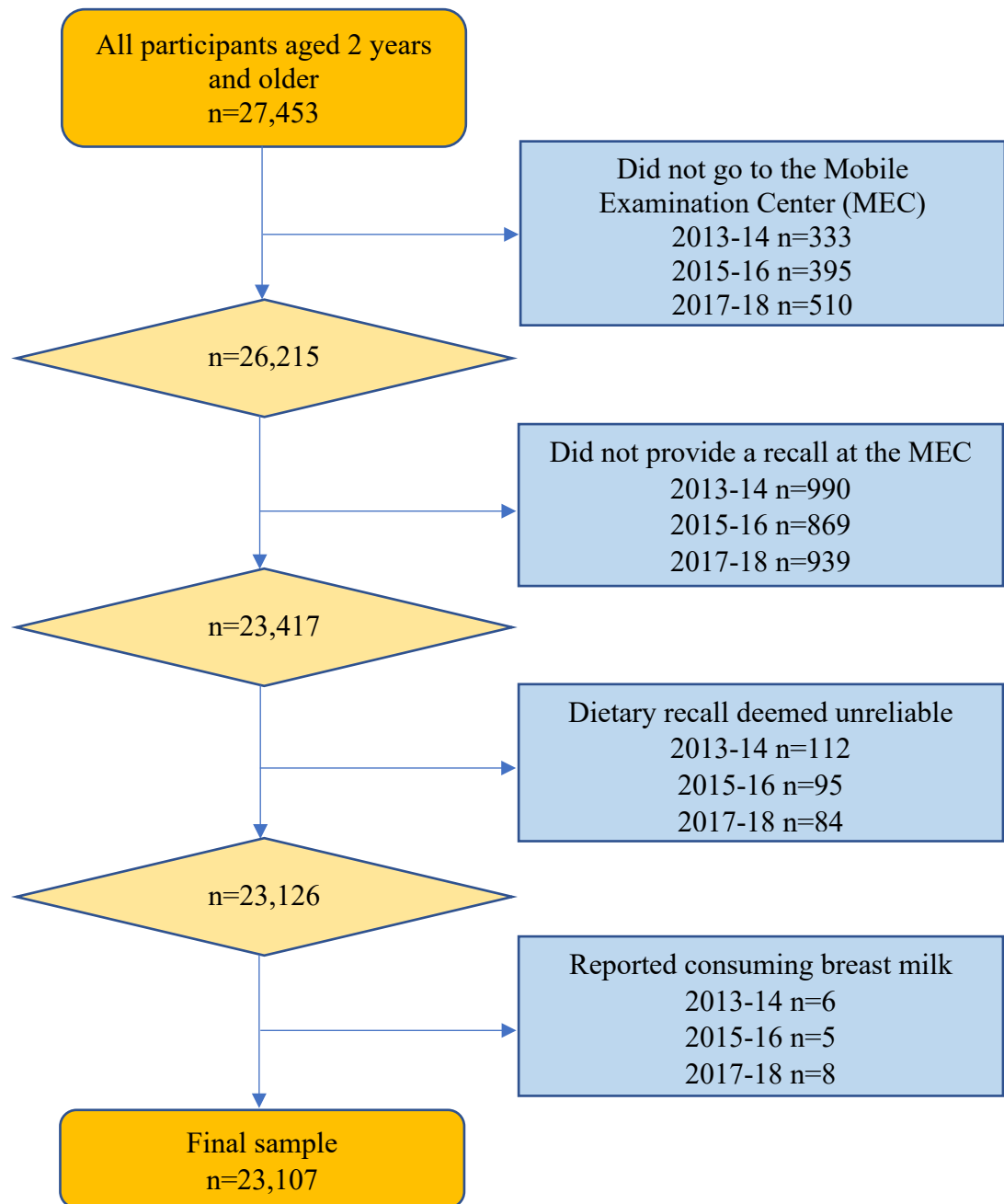
Supplementary Figure 1. Flow diagram of analytic sample, NHANES 2013-2018 1,2
