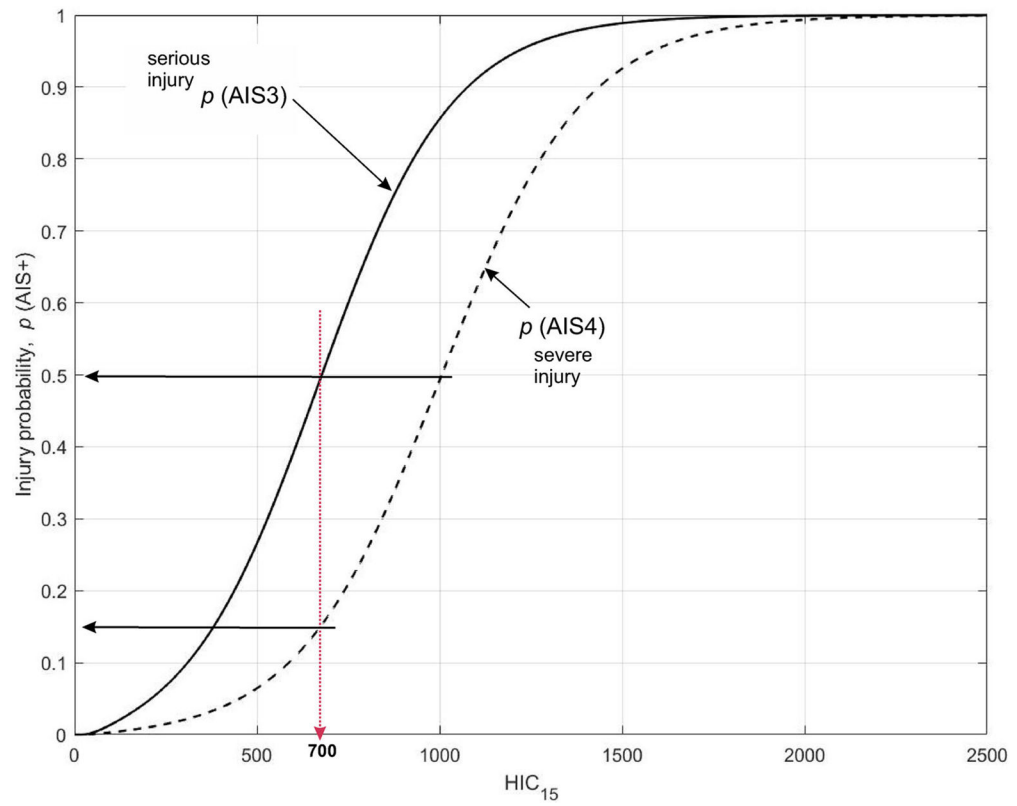
FIGURE 3. The probabilities of serious (AIS3) and severe (AIS4) injuries as a function of HIC_{15} .
