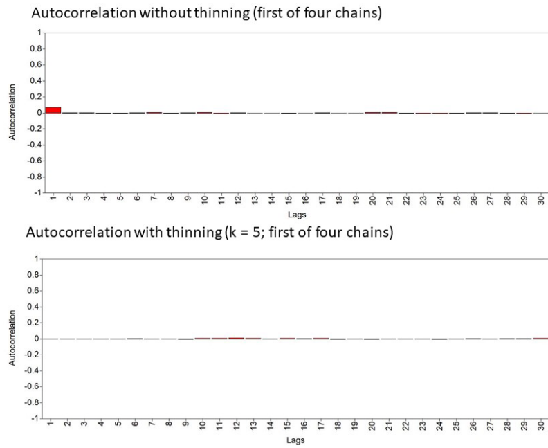
Figure S2. Autocorrelation between values of the indirect effect across iterations for one chain before and after thinning.
