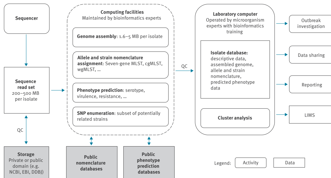
FIGURE 2 Potential solutions for computing and storage in PulseNet International laboratories, May 2017
