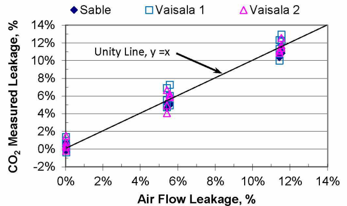
Figure 2. Air leakage test measurements made on the Clean Air Filter (CAF) Company's test stand.
