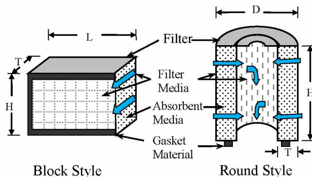
Figure 1. Carbon dioxide filter configurations (blue arrows depict airflow movement through carbon dioxide filter).
