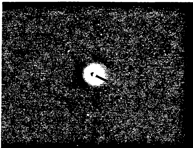
Diffraction Patterns
