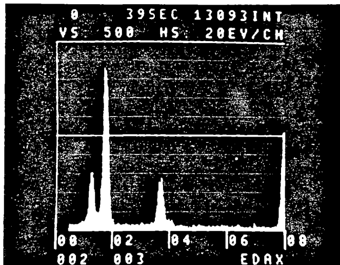
X-Ray Spectrum
