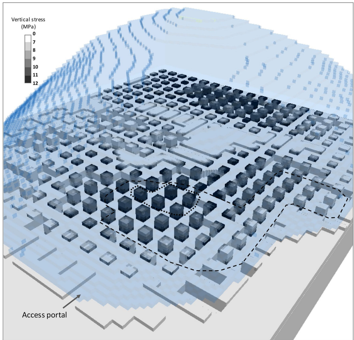
Fig. 9. Numerical model of the mine and overlying mountain shaded by the vertical stress magnitude. The collapsed area is outlined with dashed lines, and the cluster of pillars with the highest average vertical stress is outlined with a dotted line
