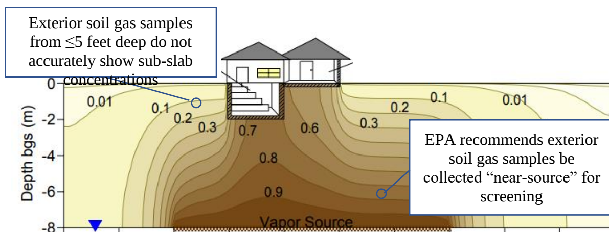
Figure 1: U.S. Environmental Protection Agency conceptual model scenario of soil gas concentrations beneath a building with a basement and a slab [EPA 2012]*
