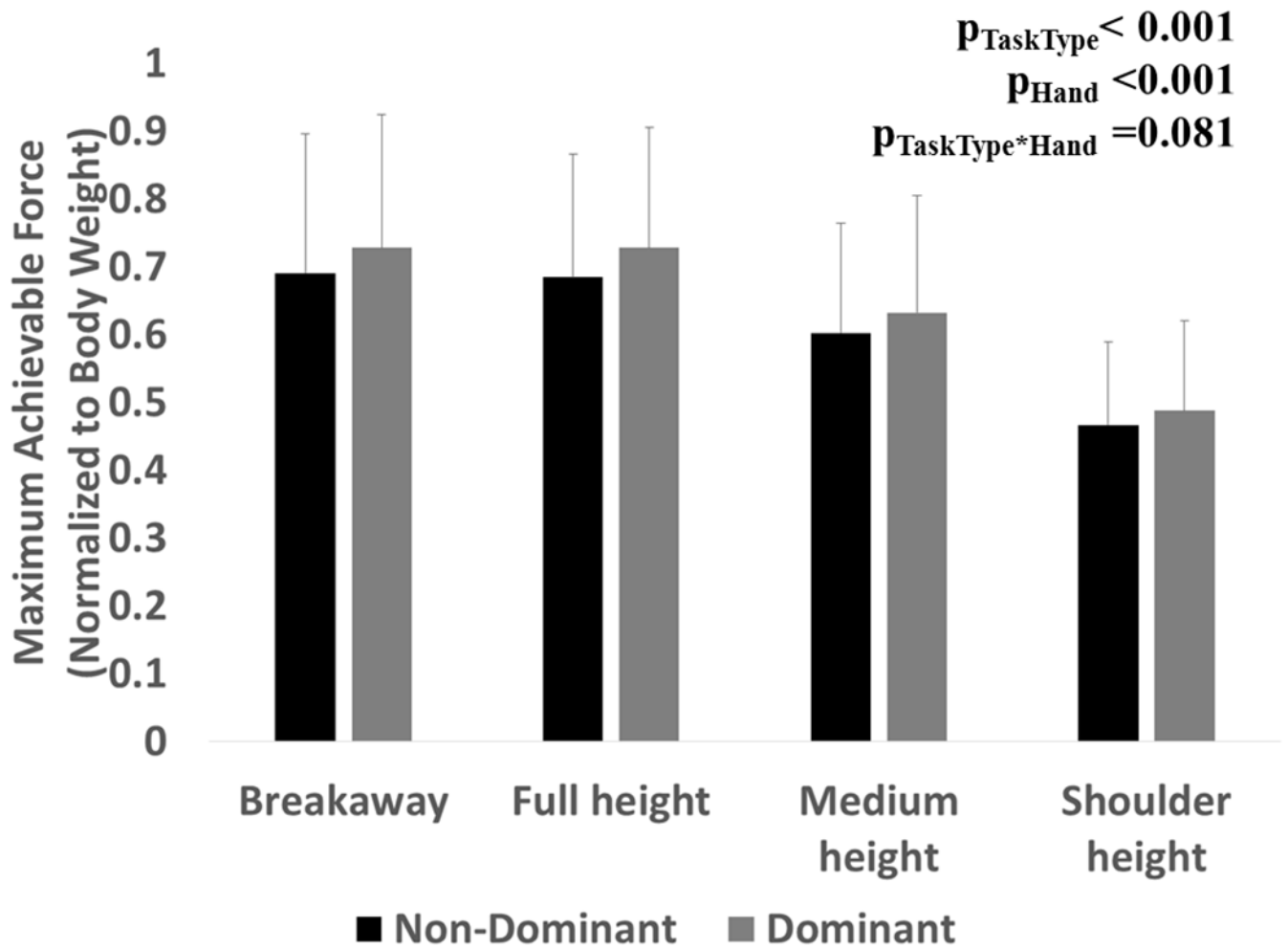
Figure 4: Impact of hand dominance and task type on the peak force that was generated. Forces are averaged across glove condition.
