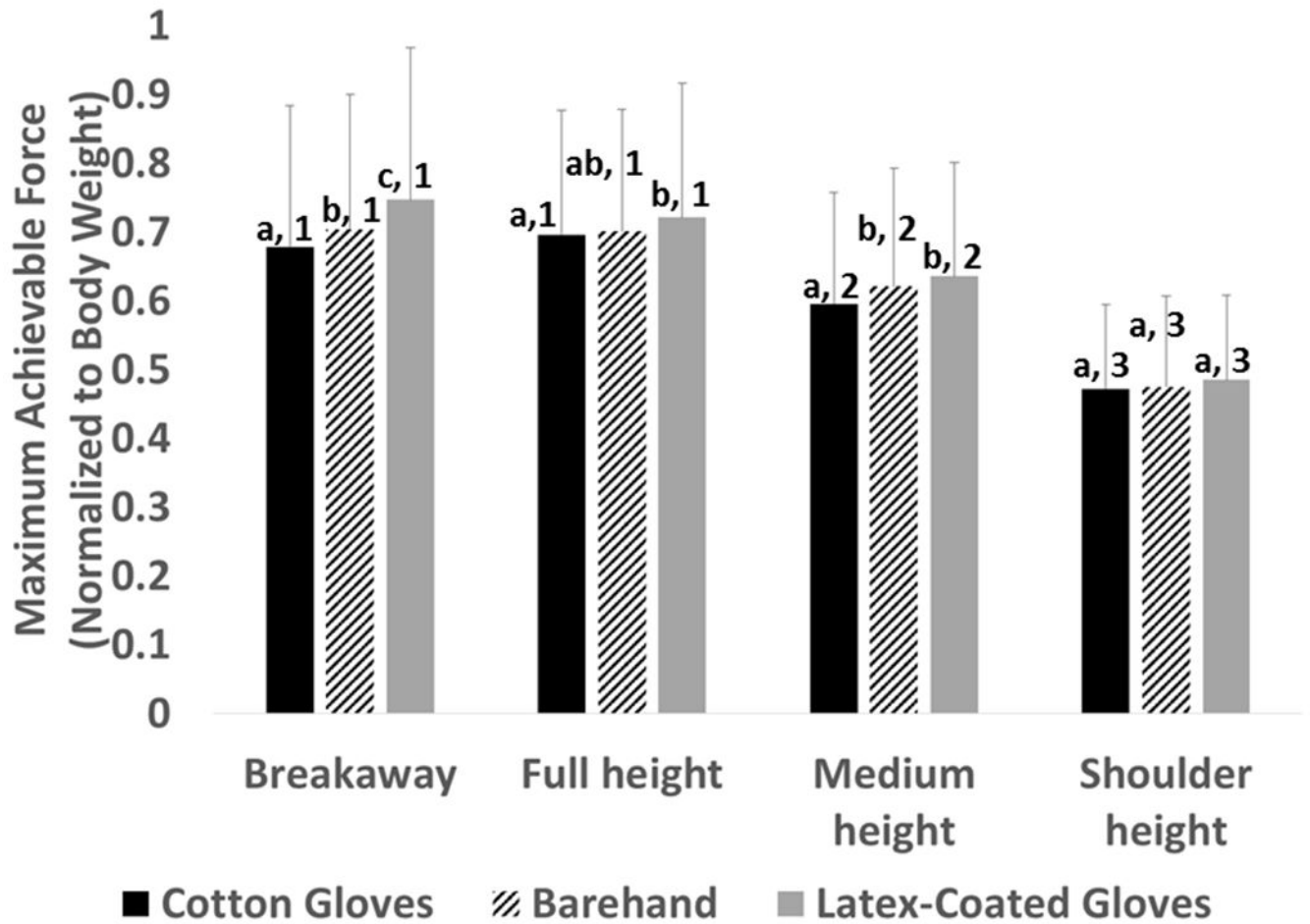
Figure 2: Impact of task and glove condition on the maximum achievable force. Error bars represent standard deviation. Numbers are used to indicate statistical significance across task type for each glove conditions. Task types with the same number are not significantly different within a glove condition. Letters are used to indicate statistical significance across gloves for each task type. Gloves that have the same letter are not significantly different within a given task. Results are averaged across the two hands.
