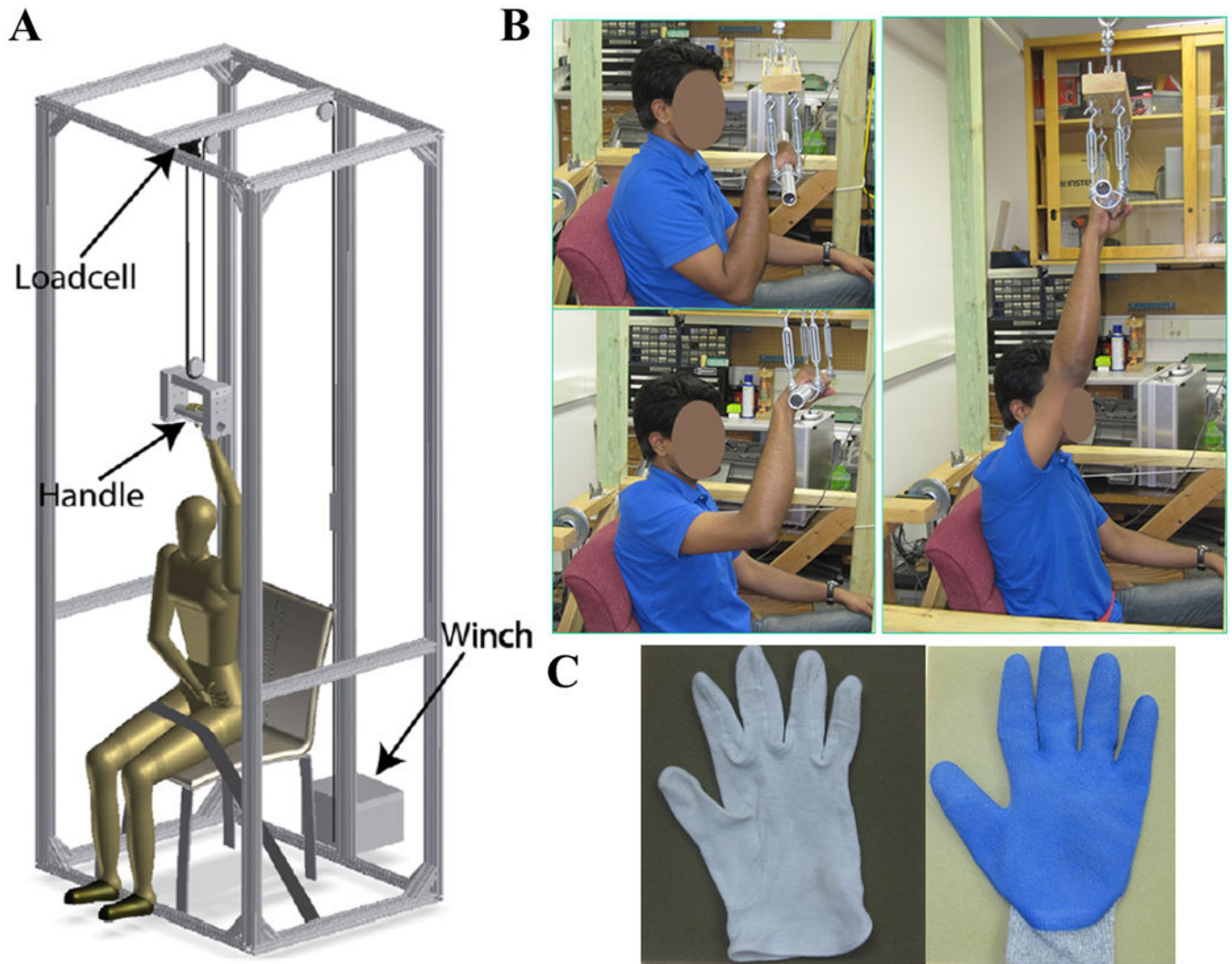
Figure 1: A) Diagram of the testing apparatus (reproduced with permission from Hur et al. (2012)). B) The three postures included in this study were shoulder height (upper left), medium height (lower left) and full height (right). C) The two glove designs used in this study included a cotton (left) and latex (right).
