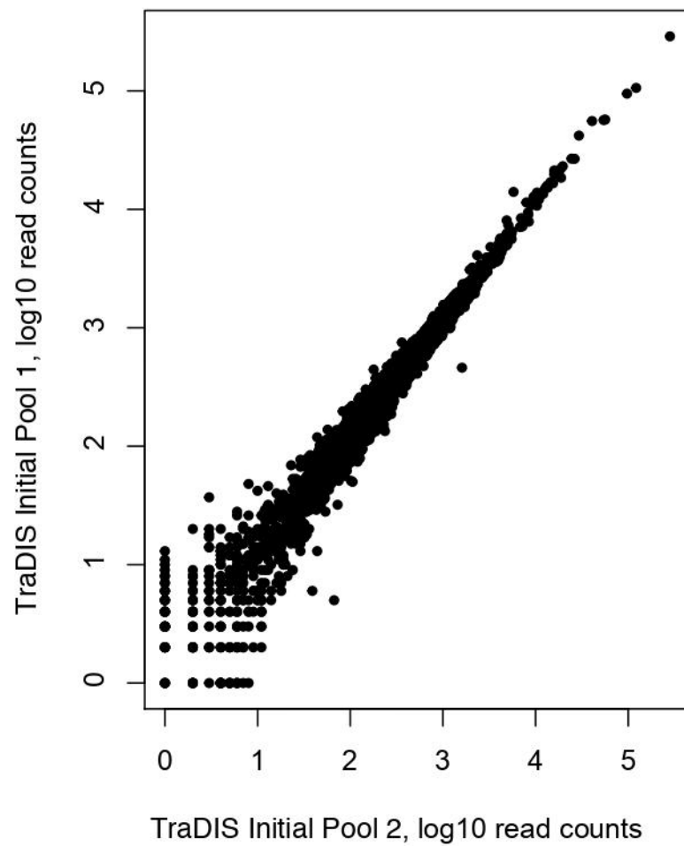
Supplementary Fig S1: Correlation coefficient of gene insertions for two sequenced biological replicates of the initial H10407 transposon library.
