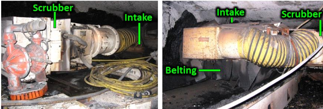
Figure 3.16. Fan-powered scrubbers with intakes at the crusher discharge (left) and stagel loader-to-belt transfer (right). Belting is hung from the transfer to further confine dust.
