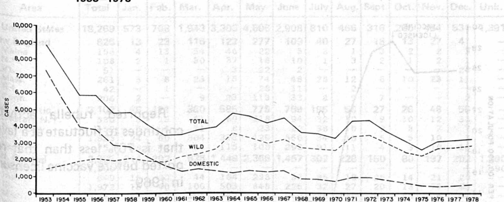
RABIES — Reported Cases in Wild and Domestic Animals by Year, United States, 1953–1978
