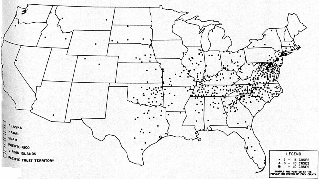
TYPHUS FEVER, TICK-BORNE (Rocky Mountain Spotted Fever) – Reported Cases by County, United States, 1978
