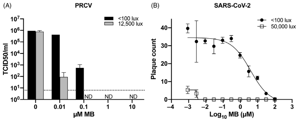
Fig. 2. Inactivation of PRCV and SARS-CoV-2 using MBL. (A) To determine the efficacy of different MB concentrations, we added serial dilutions of MB to wells of a 48-well plate containing 10 μL PRCV ( 2 \times 10^7 TCID 50 /ml). Plates were either exposed to red light (12,500 lux) for 30 minutes or were protected from light (<100 lux). The dotted line indicates the limit of detection. (B) We added serial dilutions of MB to wells of a 12-well plate containing ~50 PFU SARS-CoV-2 in MEM plus 15% FCS. Plates were either exposed to white light (50,000 lux) for 45 minutes or protected from light (<100 lux). We determined viral titers using 2–3 replicate samples. Note. FCS, fetal calf serum; MEM, minimum essential media, ND, not detected.
