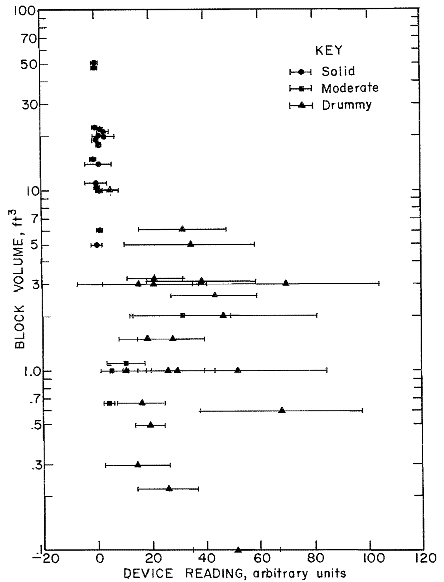
FIGURE 17. - Average device readings and standard deviations for tests performed in the CSM experimental mine.
