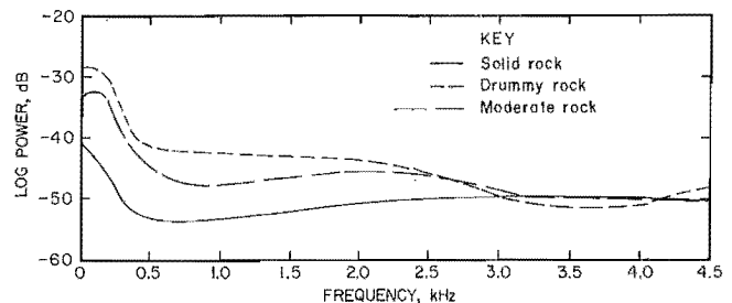
FIGURE 15. - Summary of power spectra computed for slabs tested in the Mid-Continent Resources L.S. Wood #3 Mine. Spectra are smoothed to show general behavior of the block types.
