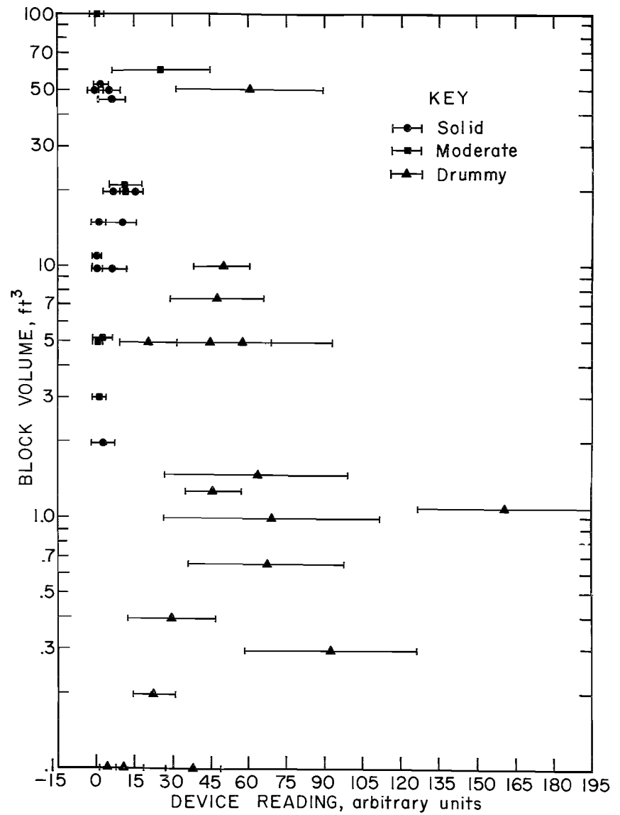
FIGURE 25. - Equivalent figure to figure 20 for the Dutch Creek #1 and L. S. Wood #3 Mines, except that gain on the differential amplifier was doubled.
