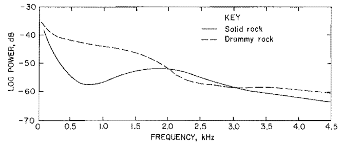
FIGURE 13. - Summary of power spectra computed for solid and drummy rocks in the CSM experimental mine. Spectra are smoothed to show the general behavior of the block types.
