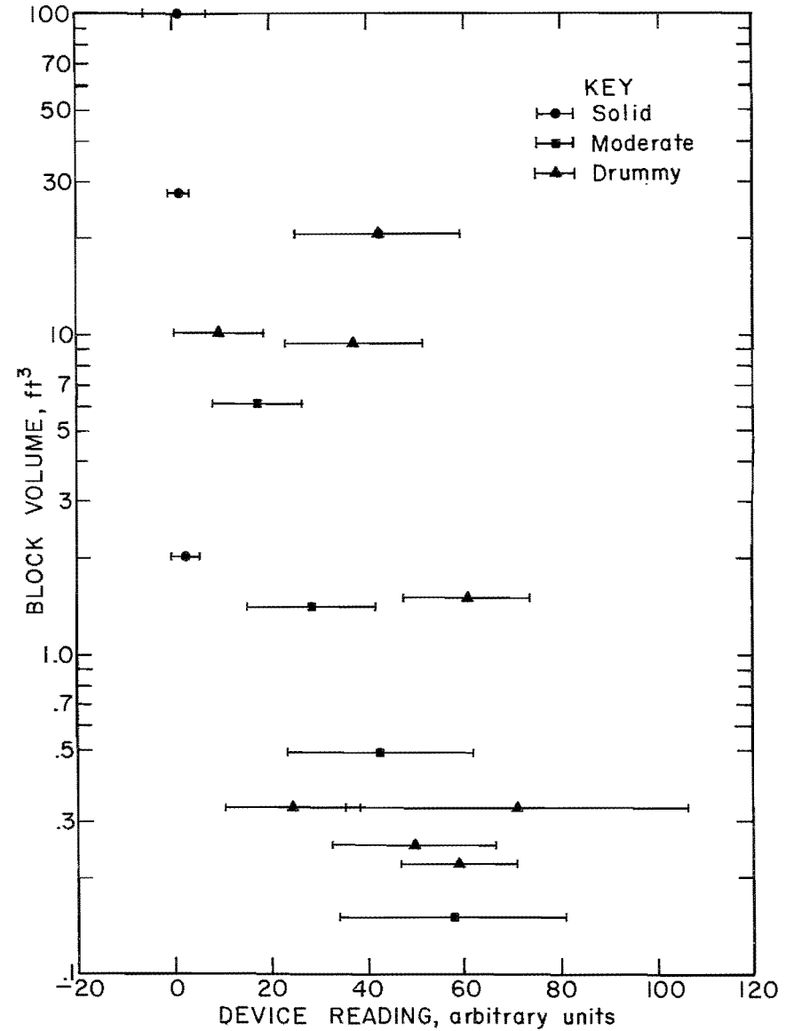
FIGURE 18. - Average device readings and standard deviations for tests performed in the AMAX Henderson Mine.
