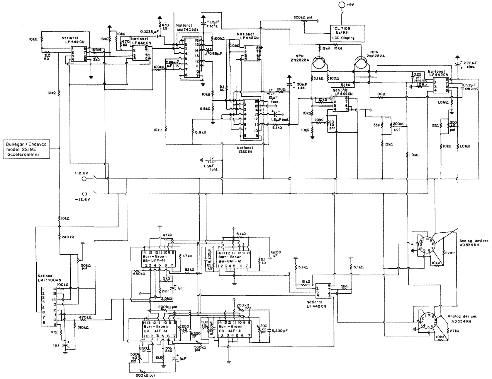
FIGURE A-1. - Schematic diagram of the current electronics circuit prototype used to measure rock slab stability based on vibrational spectrum differences.
