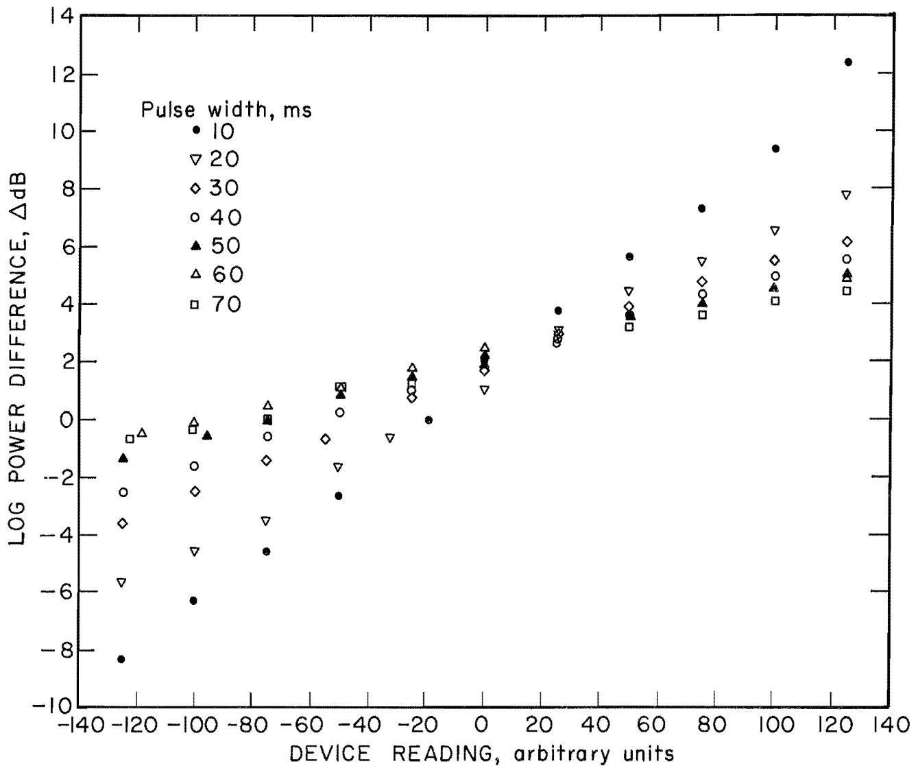
FIGURE B-1. - Calibration test on prototype. Pulse widths and amplitudes were varied to determine their relation to device reading.
