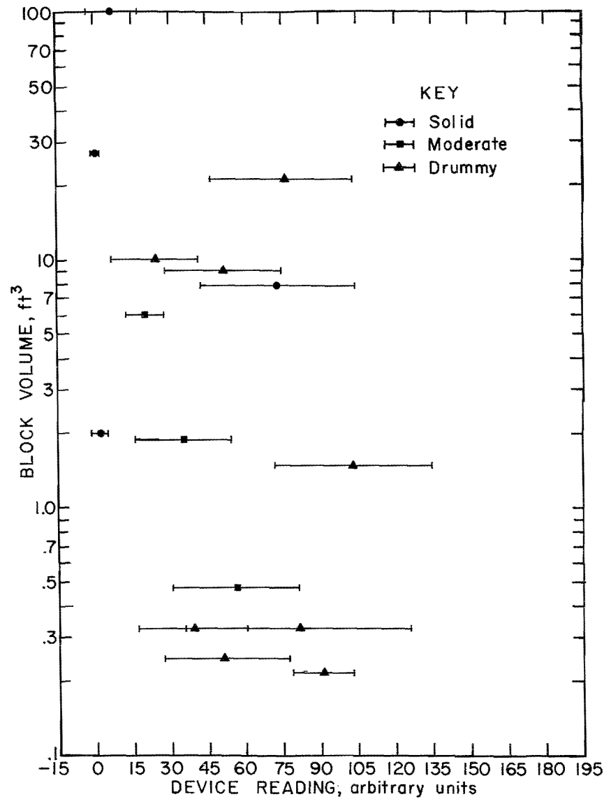
FIGURE 23. - Equivalent figure to figure 18 for the AMAX Henderson Mine, except that gain on the differential amplifier was doubled.
