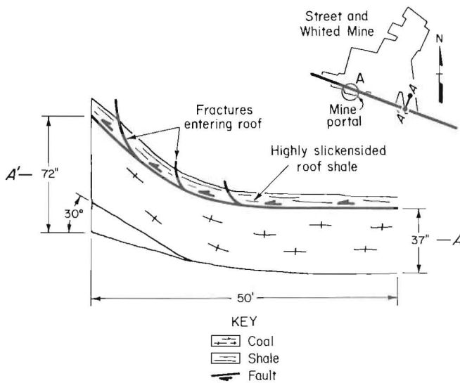
Figure 16.—Cross section of mine entry intersecting Pistol Gap Fault at Street and Whited Mine.
