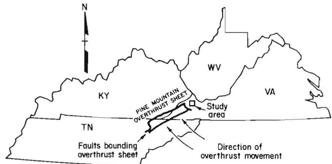
Figure 2.—Location of Pine Mountain overthrust sheet and study area.
