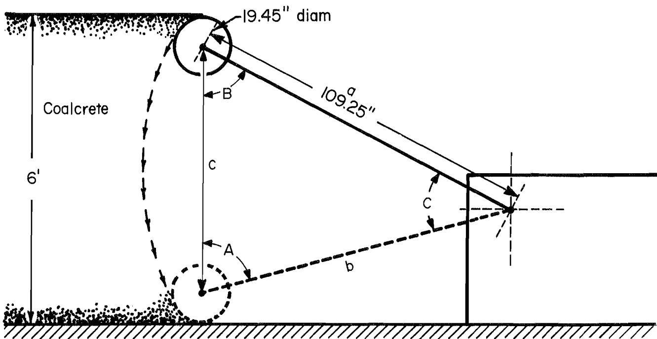
Figure B-1.—Shear angles.
