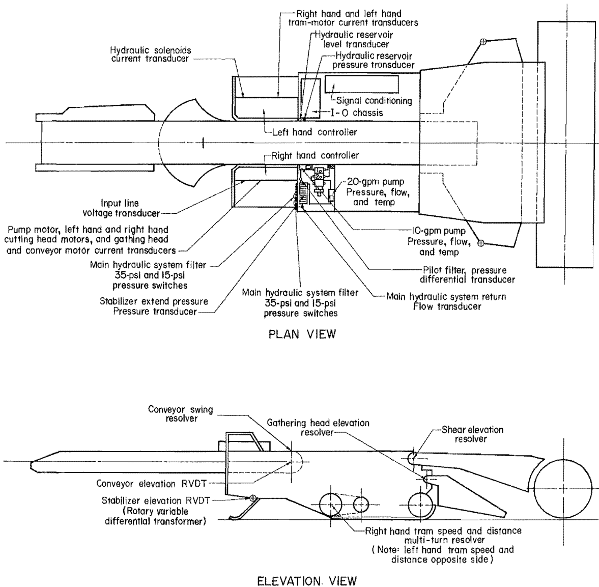
Figure 3.—Joy 16CM sensor locations.
