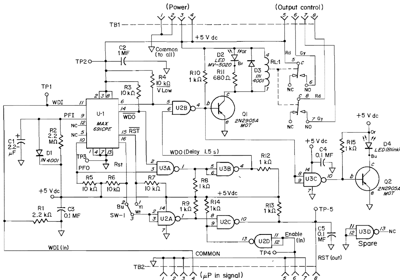
Figure 11.- Watchdog timer circuit.
