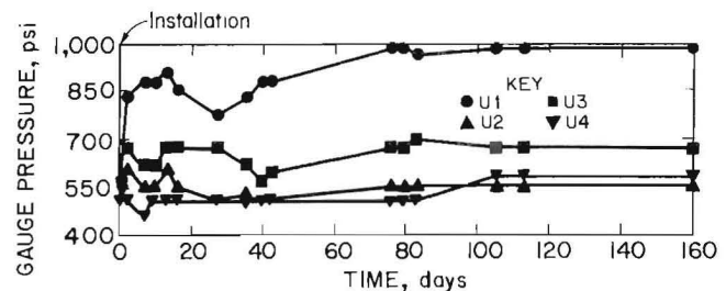
FIGURE 18.—Bolt load monitoring behavior of U-cells 1-4 (8).
