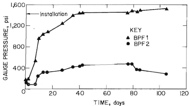
FIGURE 16.—Pressure monitoring behavior of BPF's 1 and 2 (8).
