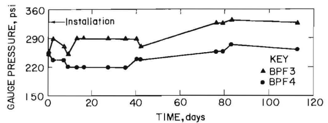
FIGURE 17.—Pressure monitoring behavior of BPF's 3 and 4 (8).
