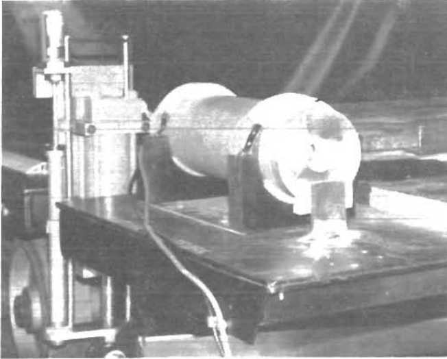
Figure 6.—Explosion-proof enclosure housing a single video camera.
