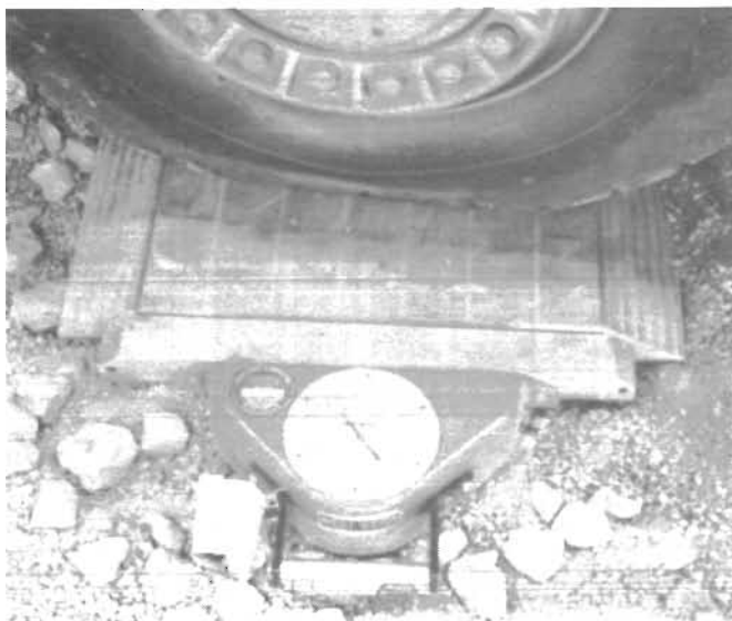
Figure 13.—Portable scales to weigh loaded, end-cab SC.
