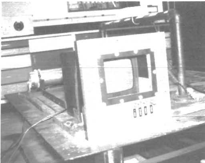
Figure 7.—Explosion-proof enclosure housing video monitor.
