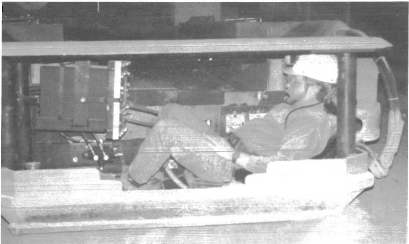
Figure 8.—Bureau-prototype end-mounted cab for low-coal SC.
