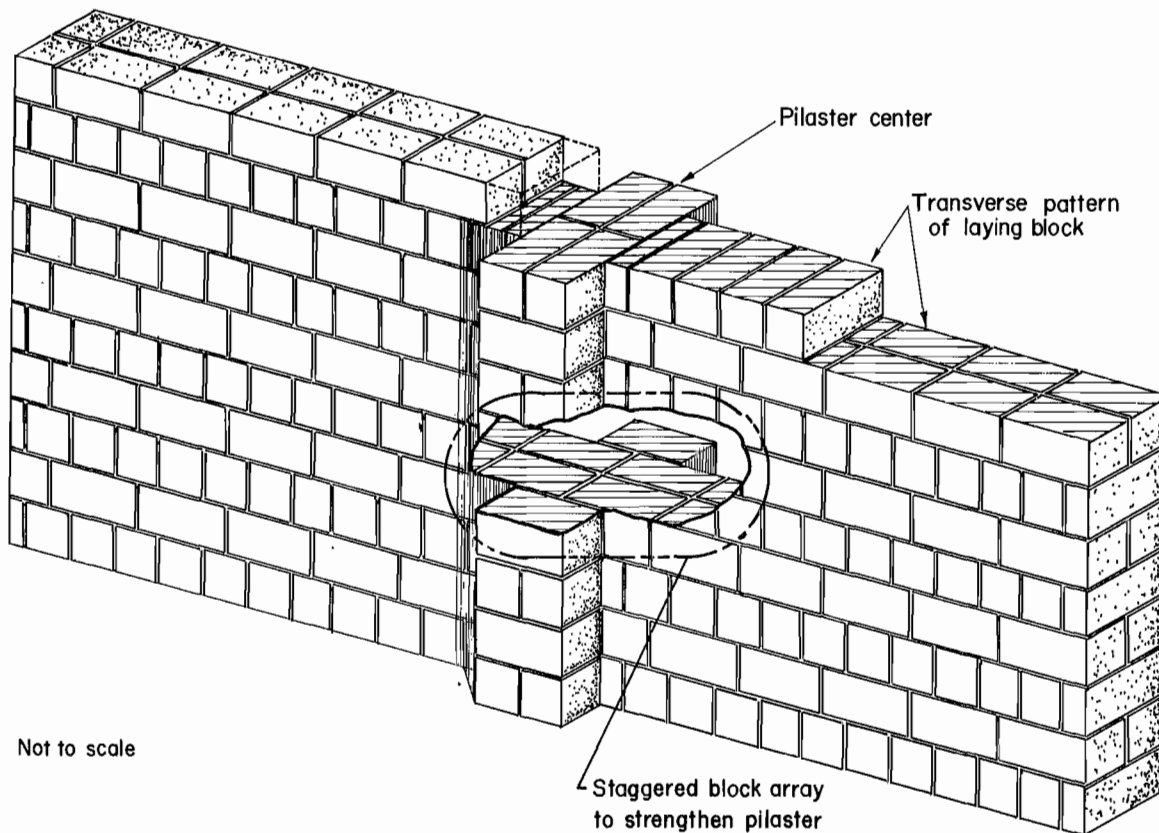
Figure 7.—Standard-type, solid-concrete-block seal.
