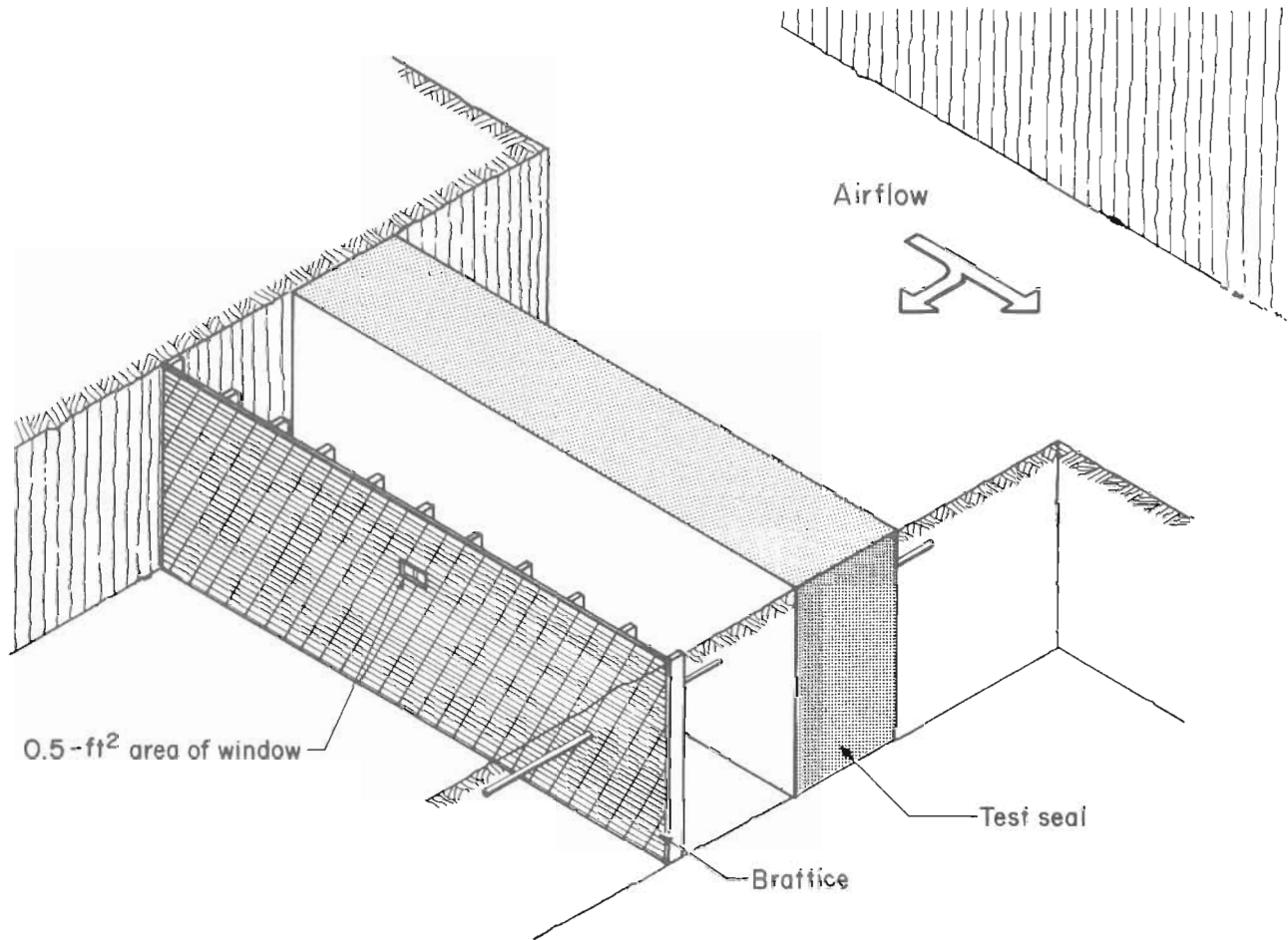
Figure 5.—Curtain configuration for leakage tests through test seal.
