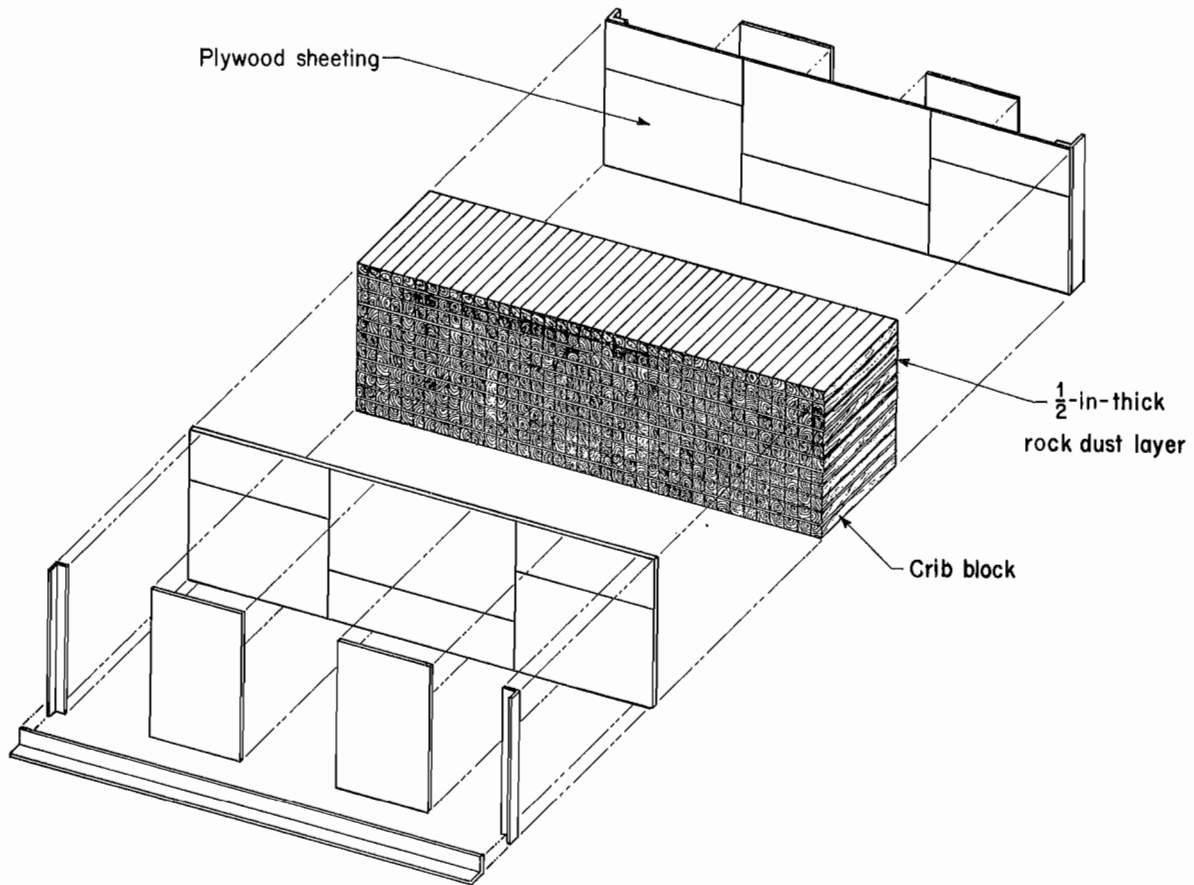
Figure 17.—Wood-block and rock-dust seal design 2.
