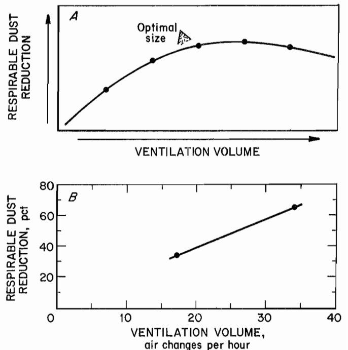
Figure 11.—Ventilation profile curves. A, Theorized ventilation profile curve with total mill ventilation system; B, ventilation profile curve for mill 2.
