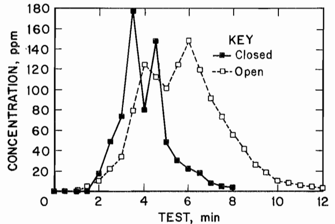
Figure 10.— \text{SF}_6 analysis—effectiveness of total mill ventilation system with windows open versus closed. Concentrations recorded at east fan.
