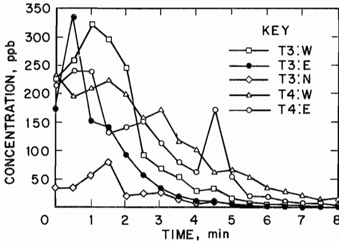
Figure 9.— \text{SF}_6 analysis—comparing four fans (T3) versus two fans (T4) for total mill ventilation system. W, concentration recorded at west fan; E, concentration measured at east fan; N, concentration recorded at north fan.
