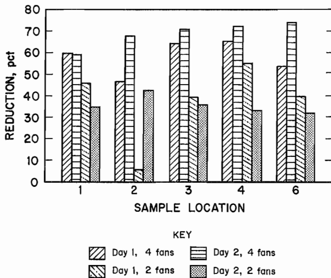
Figure 6.—Percent reduction of respirable dust at each monitoring location for 2 days of testing for both two and four fans using RAM-1 devices.
