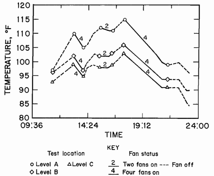
Figure 7.—Temperature readings at three levels in mill building during day 1 of testing with and without total mill ventilation system.
