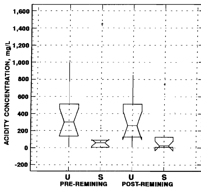
Acidity concentration medians of underground (U) and surface (S) mines before and after remining.
