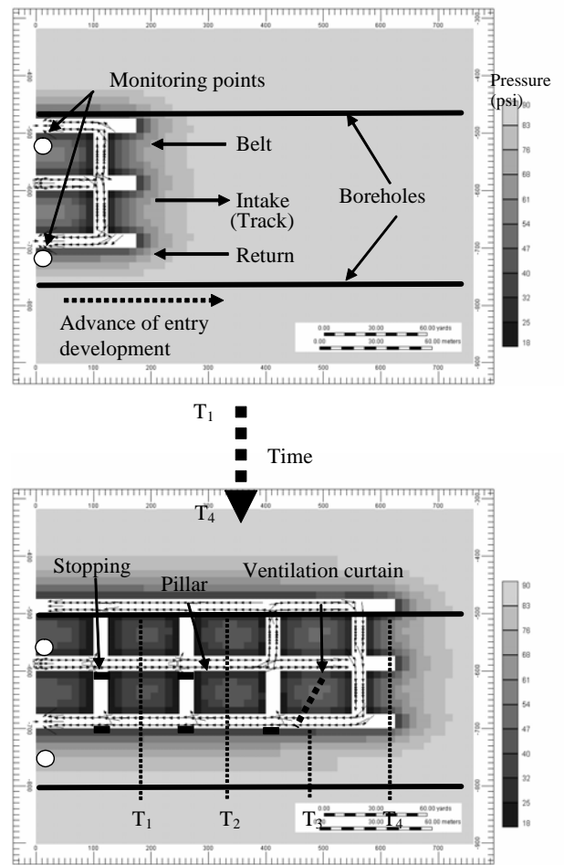
Figure 2. Snapshots of mining advance, pillar layout, and the ventilation scheme in the coalbed reservoir model. Locations where total methane inflow is monitored are also shown. The figures show the progress of mining in the coalbed at the end of first and fourth section advances.
