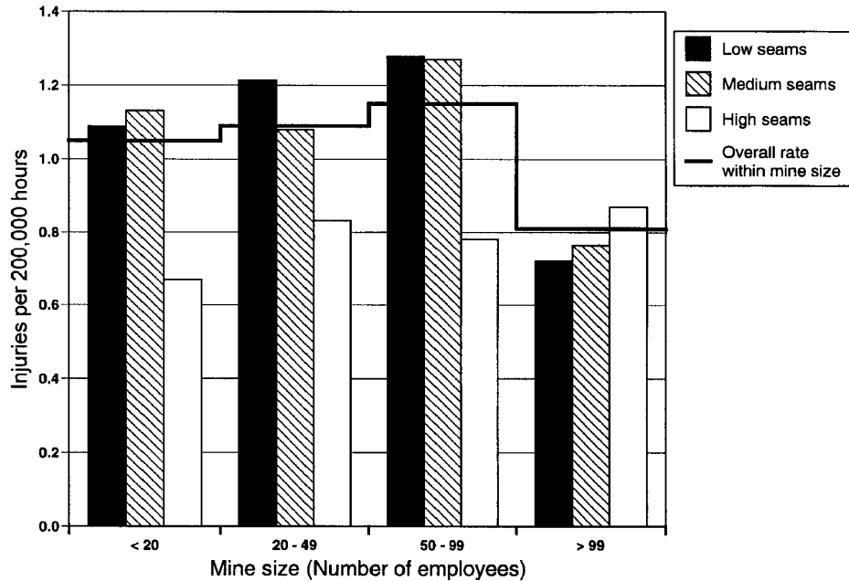
Figure 16.—Rate of nonfatal disabling injuries from roof bolting machinery accidents by mine size and seam height, 1990-94.
